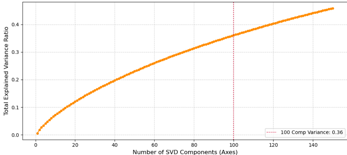
SVD Scree Plot: Cumulative Explained Variance vs. Components
